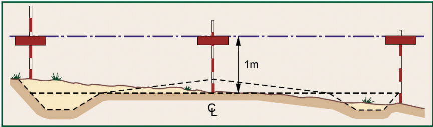
Figure 25: Transfer level from the profile board at center line to the outer ranging rods
