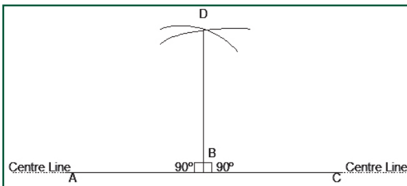
Figure 11: Setting out a right angle by string
