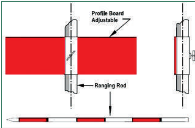
Figure 2: Profile board and ranging rod
